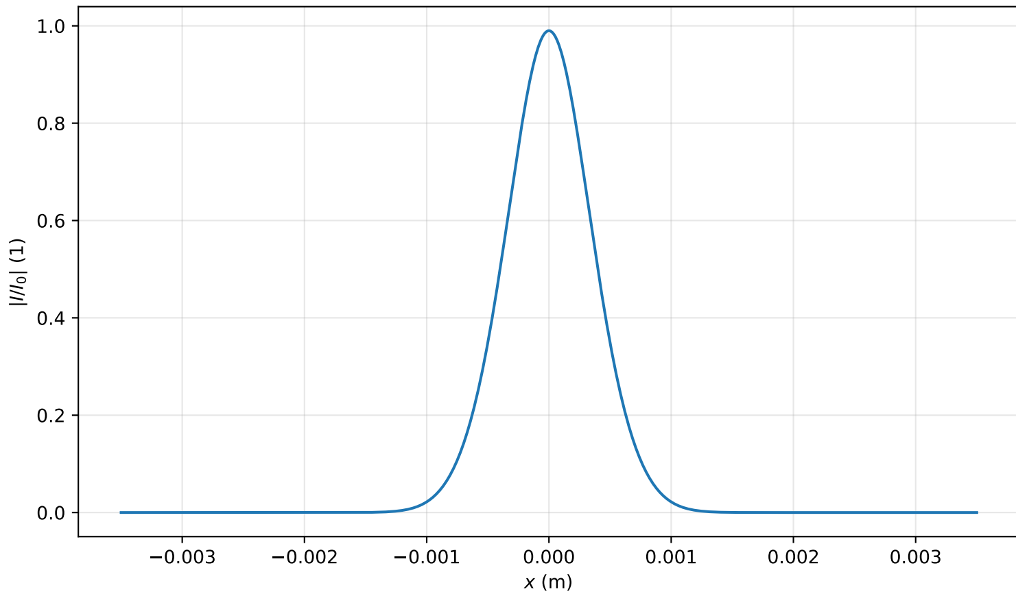
Intensity profile I(x, y = 0, z = 0.637m)/I_0 , P_{in}=0.3P_{cr} , artificial time
